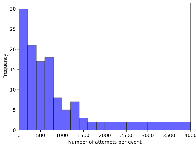
Fig. 4.2: Typical distribution of the number of attempts it takes for the existing 2D generator before the test direction gets accepted, per event.
