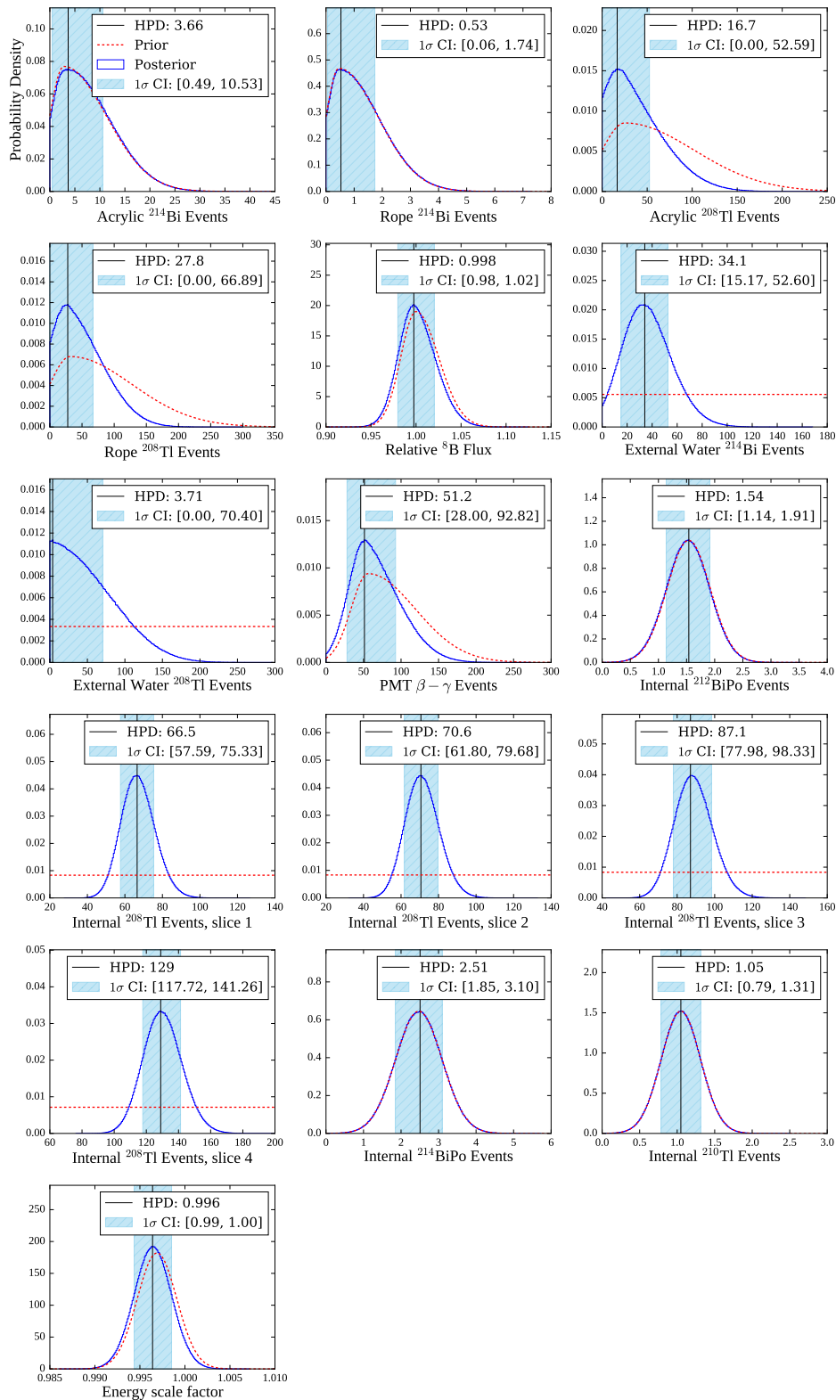
Fig. 6.17: Marginalised 1D posterior density distributions for all non-oscillation parameters, shown in blue. The HPD and 1\sigma Bayesian CI are shown for each parameter. Also shown in dashed red are the associated prior distributions.
