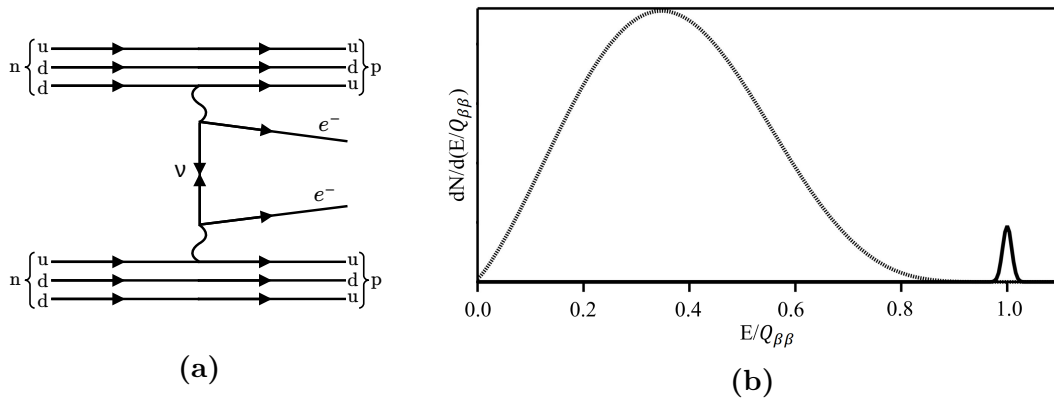
Fig. 1.7: (a): Feynman diagram for 0\nu\beta\beta decay. (b): Sketch of the energy spectra for 2\nu\beta\beta (dashed line) and 0\nu\beta\beta decays (solid line). The Q -value of the decay is written here as Q_{\beta\beta} . Taken from [79].
