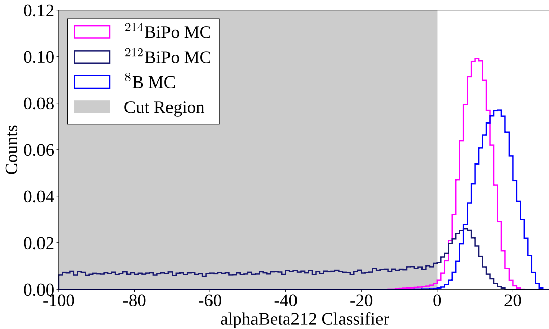
Fig. 6.7: The distributions of the IW ^{212}\text{Bi} -Po classifier for Bi-Po and ^8\text{B} events in simulation, within the analysis ROI. The cut of alphabeta212 < 0 clearly removes a large fraction of ^{212}\text{Bi} -Po events, and 2% of ^{214}\text{Bi} -Po events, while keeping 99.89% of the ^8\text{B} signal. The relative normalisations before these cuts have been applied is arbitrary.
