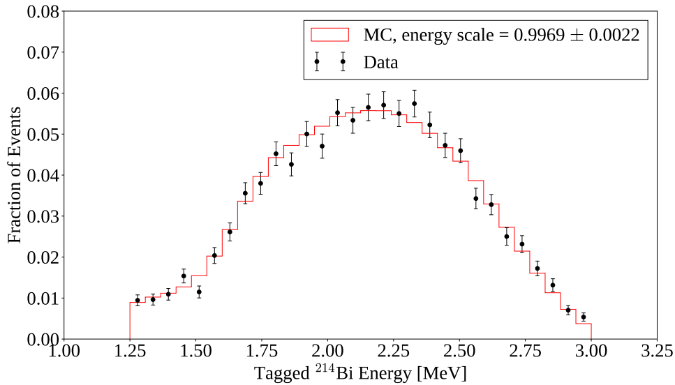
Fig. 6.15: Comparison of tagged ^{214}\text{Bi} reconstructed energy distributions between data and MC, after MC has been scaled by the best-fit factor \alpha = 0.9969 .
