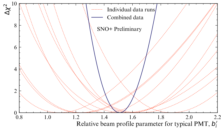
Fig. 4.6: Plot of \Delta\chi^2 \simeq X_i , twice the negative log-likelihood ratio, for both single subruns of a typical PMT, and when all relevant subruns are combined.
