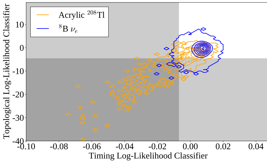
Fig. 6.12: Distributions of the timing and topological external classifiers, for both the {}^8\text{B} signal and {}^{208}\text{Tl} decays in the acrylic. Contours indicate lines of equal probability density. All events shown were in the analysis ROI, and below 5 MeV. Grey regions indicate the cuts used in this analysis.
