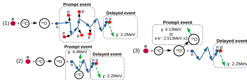
Fig. 6.9: Schematic of the three dominant modes of (\alpha, n) interaction, taken from [90].
