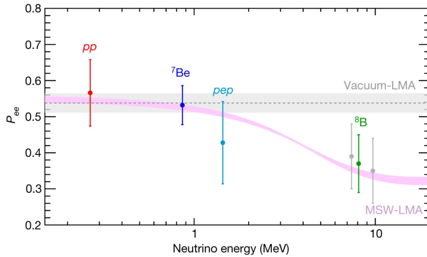
Fig. 1.5: Measured survival probability versus mean neutrino energy for each solar neutrino type, as observed by Borexino. Taken from [29]. For comparison, the expected survival probability due to vacuum oscillations and the MSW effect are shown as grey and pink bands, respectively.
