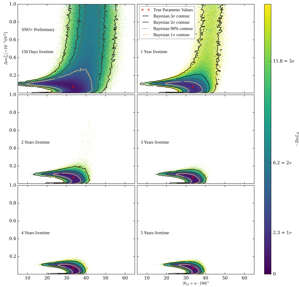
Fig. 6.22: Posterior density distributions marginalised onto the two solar oscillation parameters, for each livetime scenario in the pure scintillator phase under the current backgrounds.
