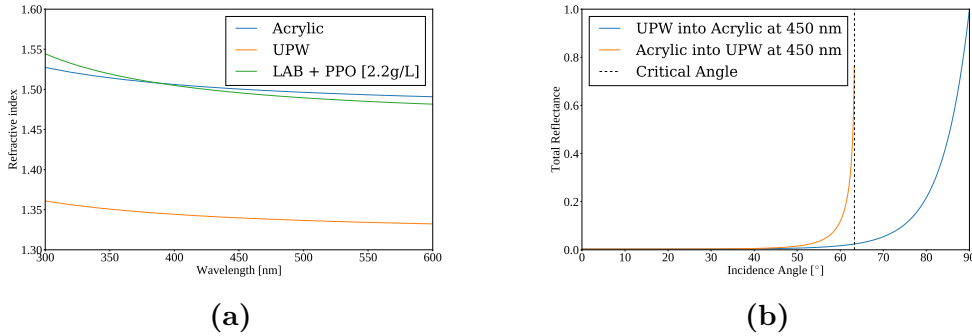
Fig. 2.6: (a): Refractive indices of acrylic, UPW, and LAB-PPO as a function of wavelength. The values for acrylic and UPW come from model fits to data made in SNO [114, 122], whereas those for LAB-PPO come from data taken in [123]. (b): Reflectance of an unpolarised beam of light at 450 nm going between UPW and acrylic.
