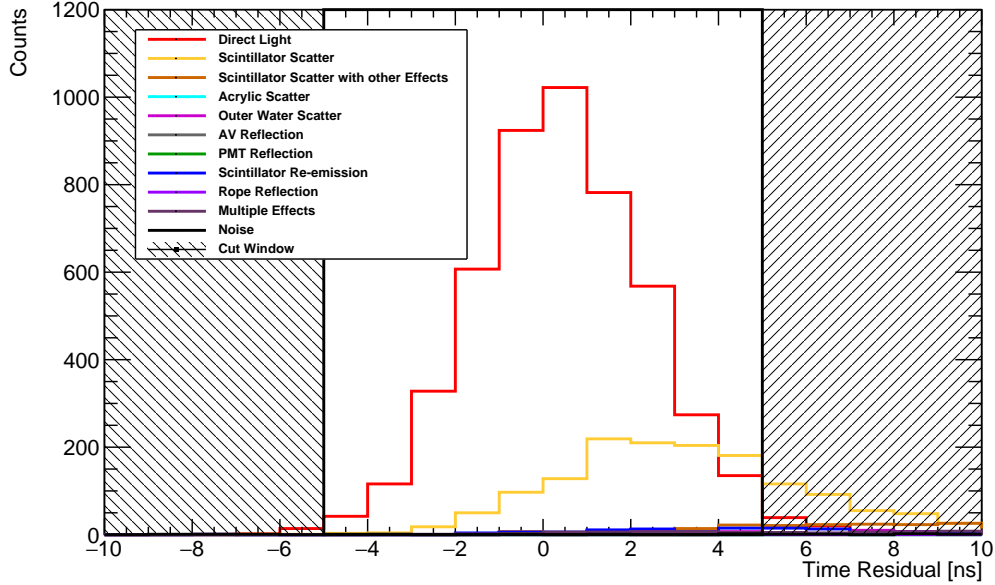
Fig. 5.7: Far PMT time window selection applied to a simulation of the PQ407 laser fired through laser FS107. The substantial background contribution from scattered light can be seen.
