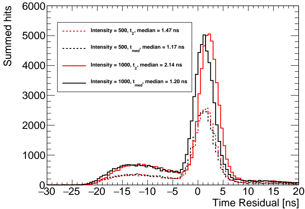
Fig. 5.5: Comparison of the backscatter light region time residual distribution, as a function of both emission intensity and emission time calculation choice. A clear intensity-dependence can be seen when using t_2 , whereas t_{\text{med}} is much more robust.
