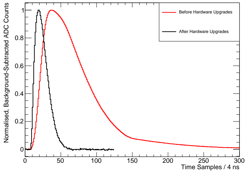
Fig. 3.12: Comparison between typical MPU CAEN traces generated by the PQ495 before and after the Summer 2022 hardware upgrades. The data before was taken on July 24 th 2022, whilst the data after was taken on June 17 th 2023. The traces have had their baselines subtracted off, and their peak values normalised to 1.
