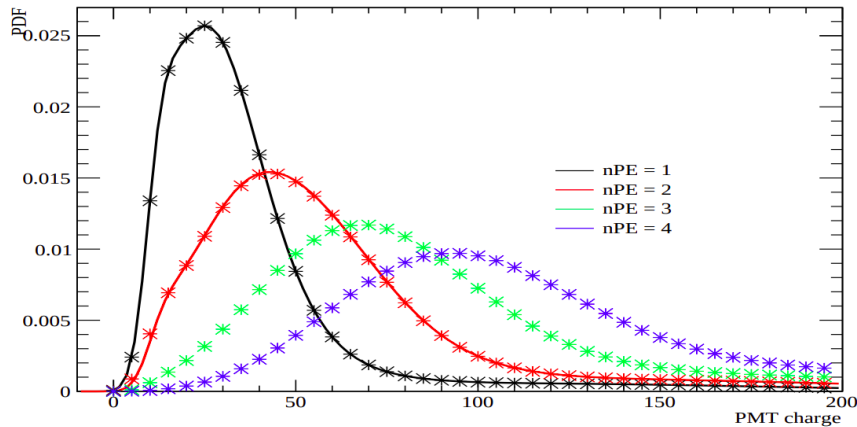
Fig. 2.9: Example charge spectra for a PMT as a function of the true npe generated. Figure taken from [127].
