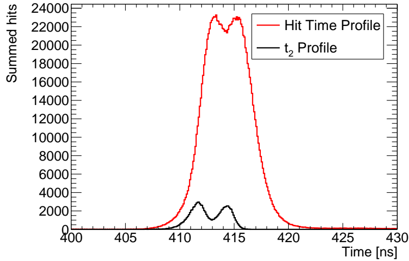
Fig. 3.14: Hit time and t_2 distributions for a subrun of SMELLIE data taken with the SuperK laser in the [490, 500] nm range through fibre FS125 on June 17 th 2023. The double-peaked structure is clear in both distributions.
