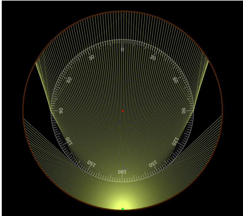
Fig. 5.13: Model of light rays propagating in the SNO+ detector during scintillator phase, emanating from an external source such as SMELLIE. Because of refraction, a large ringed region is formed where no direct light can reach the region from the source. This forms the basis of the new scattering signal region.
