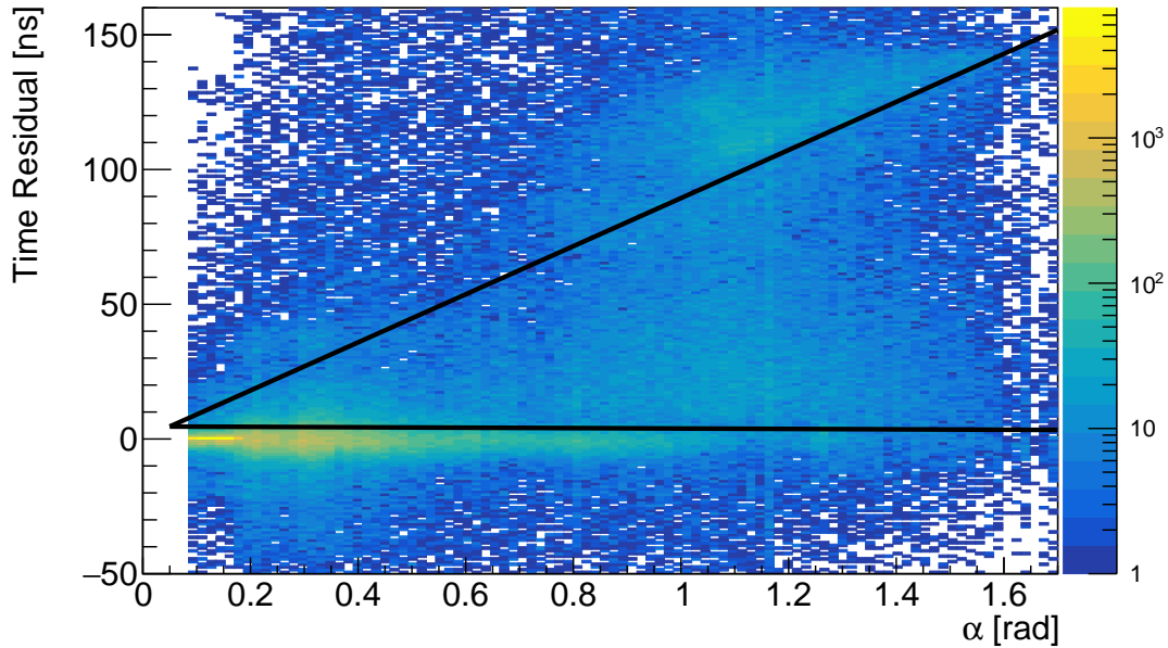
Fig. 5.12: Hit distribution of data taken in run 302,634, with laser PQ495 through fibre FS055, as a function of both t_{res} and \alpha . The triangular scattering signal region optimised from Fig. 5.11a.
