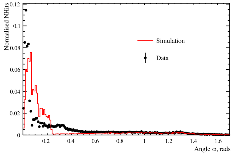
Fig. 4.1: Comparison between a simulation of one of the fibres, made from the 1D beam profile generator (red), with the associated data subrun that was used to create that beam profile (in black). For both MC and data, what is plotted is the PDF of observed PMT hits, as a function of the \alpha angle. Poissonian errors have been added to the data points, but are too small to see. Clearly, this 1D generator does not replicate the observed beam profile correctly. Figure taken from [115].
