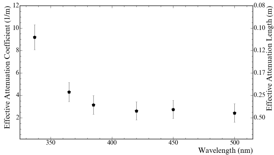
(b) Acrylic optical attenuation
