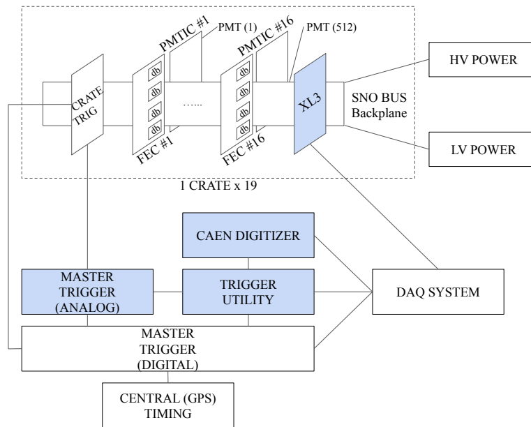
Fig. 2.10: Schematic of the front-end electronics used for data acquisition and triggering in SNO+, taken from and discussed in [84].
