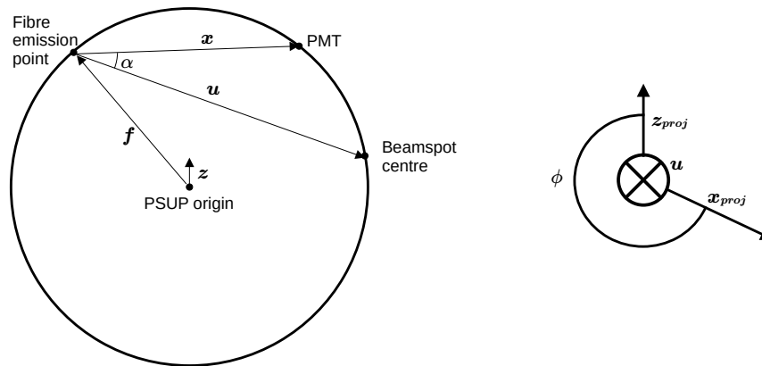
Fig. 3.11: Diagram of the SMELLIE coordinate system, adapted from [115]. The right-hand drawing is being shown in the plane orthogonal to \hat{u} .
