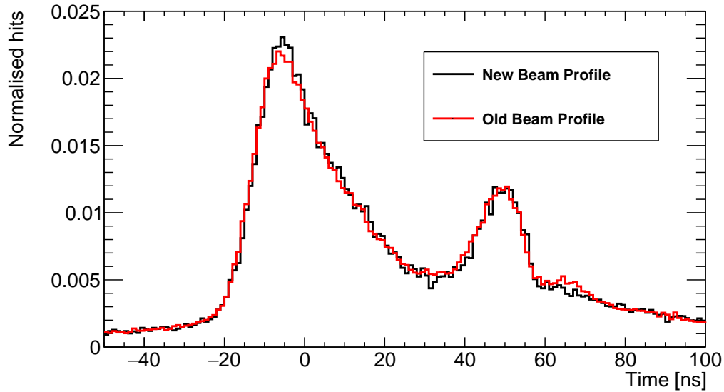
Fig. 5.15: Comparison of timing distributions in the bad light-path PMT region for simulations of laser PQ495 through fibre FS055, comparing the old and new beam profile. Both distributions have been normalised by the number of events. The fractional difference in the number of hits in the signal time window is 1.0%.
