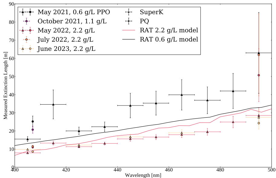
Fig. 5.10: Summary of scintillator extinction length measurements made by SMELLIE, with a comparison to the current 2.2 g/L optics model used in RAT.
