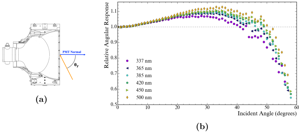
Fig. 2.7: (a): Diagram of the PMT and concentrator ‘bucket’ used within SNO+, showing also the definition of the incidence angle. (b): Plot of the measured relative angular response of the PMTs in SNO+, as a function of both incidence angle and wavelength. Both figures taken from [85].
