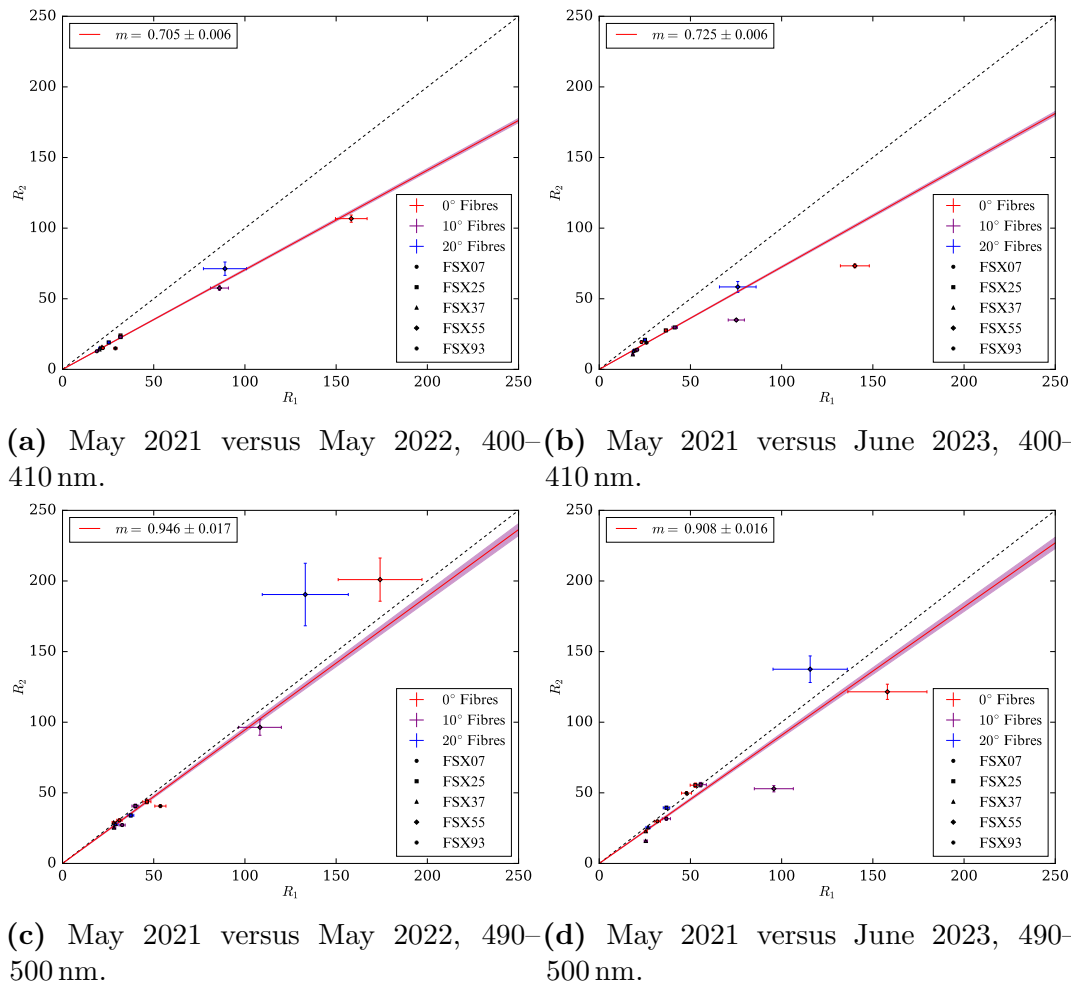
Fig. 5.16: Plots of R_1 against R_2 for four pairs of scintillator phase datasets, using the SuperK laser.
