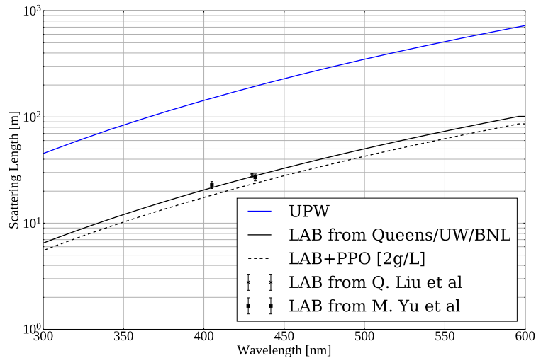
Fig. 2.4: Scattering lengths used in simulation for UPW, LAB, and 2 g/L LAB-PPO. The UPW shape is taken from indirect in-situ measurements in [114] with an additional divisive scaling factor from [115]. The LAB shape is taken from ex-situ measurements by SNO+ members at Queen’s University, University of Washington, and Brookhaven National Laboratory [116, 117]. An additional divisive scaling factor of 1.176 due to PPO was made by [118]. For comparison, measurements by members of the JUNO Collaboration for LAB are also shown [119, 120].
