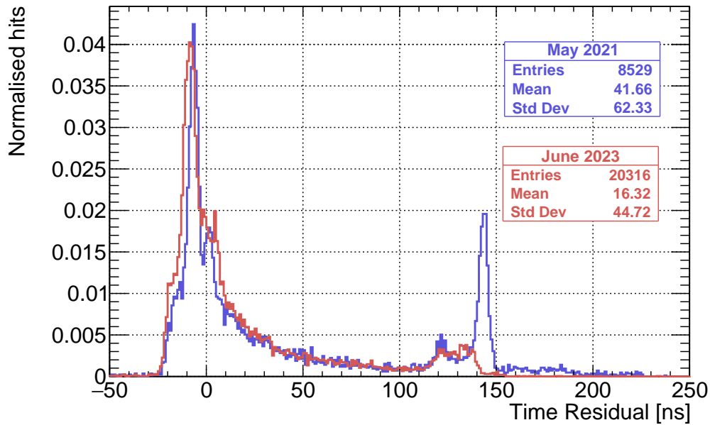
Fig. 5.18: Observed time residual distributions for the backscattered light region of PMTs, with the SuperK laser in the 490–500 nm range through fibre FS037. The distributions from both May 2021 and June 2023 are compared, with both of their distributions normalised to 1. The lack of the peak at 145 ns in the June 2023 data likely comes from the changing of the TUBii trigger delay during the hardware upgrades of Summer 2022: see Section 3.5 for more details.
