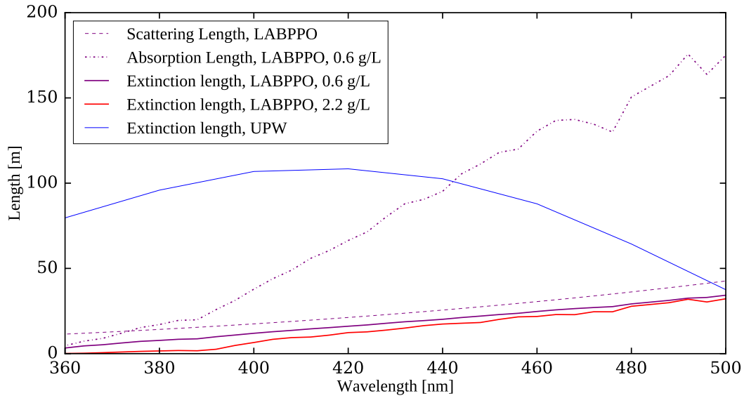
Fig. 5.1: Current RAT models for the extinction lengths of both UPW and scintillator, at different PPO concentrations as a function of wavelength. For the scintillator, the absorption and scattering length distributions are also shown as a dotted line, showing that it is expected for scattering to dominate over absorption in the 400–500 nm range.
