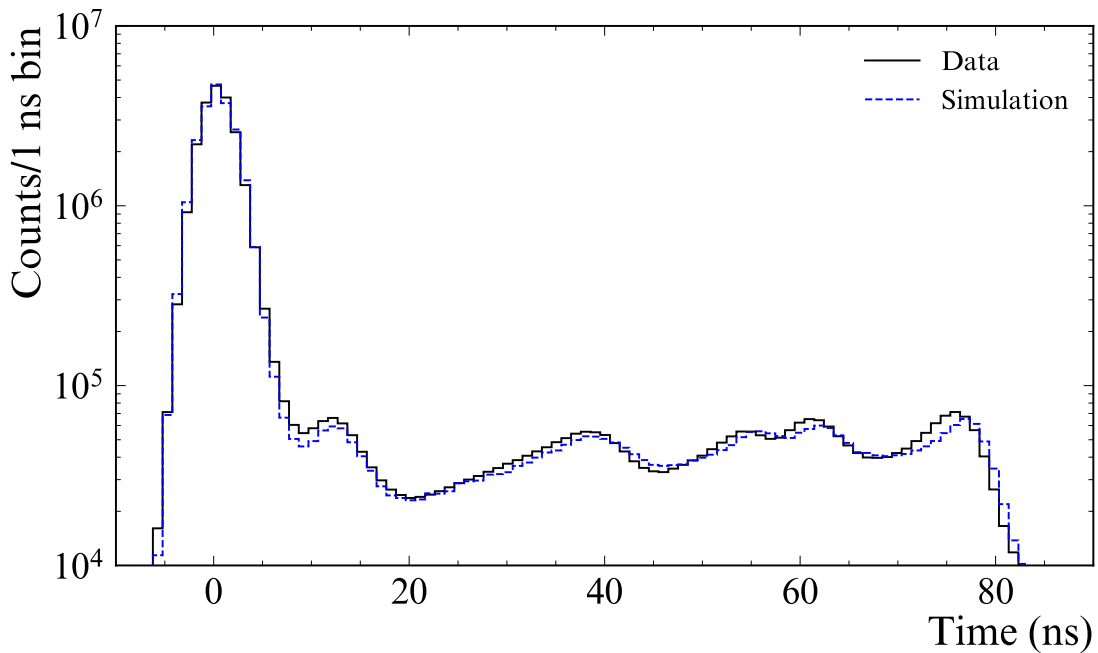
Fig. 4.12: Comparison of Laserball data in the water phase to MC, with a wavelength of 420 nm. The latest peak comes from PMT reflections. From [85].
