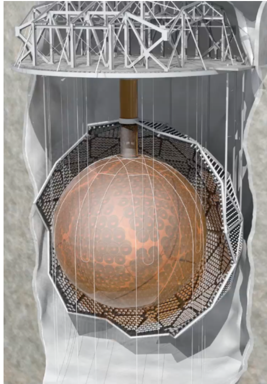
Fig. 2.1: 3D model of the SNO+ detector [84].
