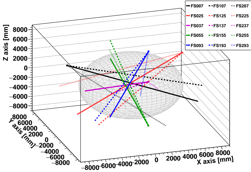
Fig. 3.10: Fibre emission points and nominal pointing directions within the detector.
