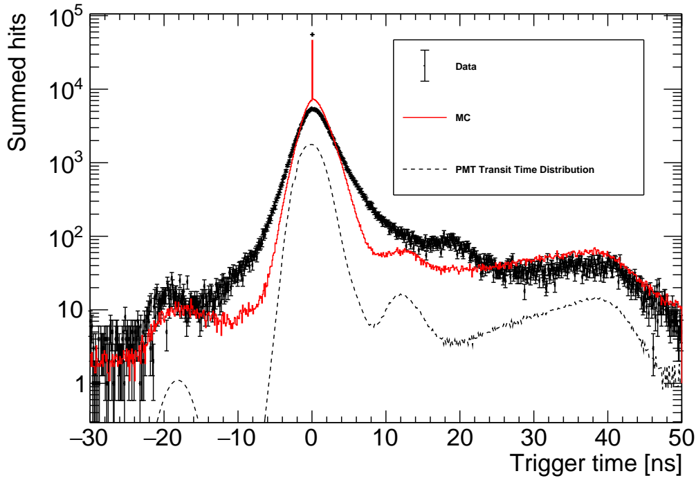
Fig. 4.10: Time residual distribution in the beamspot region for data taken in July 2022 with PQ495 through fibre FS007, as compared to a matching simulation. Also shown is the PMT transit time distribution, taken from [148]. The width of the data’s prompt peak is much broader than expected, and there is a notable bump at 19 ns not present in the MC or the PMT transit time distribution.
