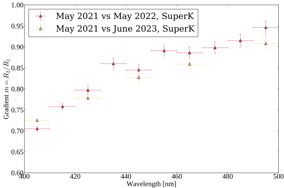
Fig. 5.17: Summary of results from the scattering analysis, shown as a function of wavelength.
