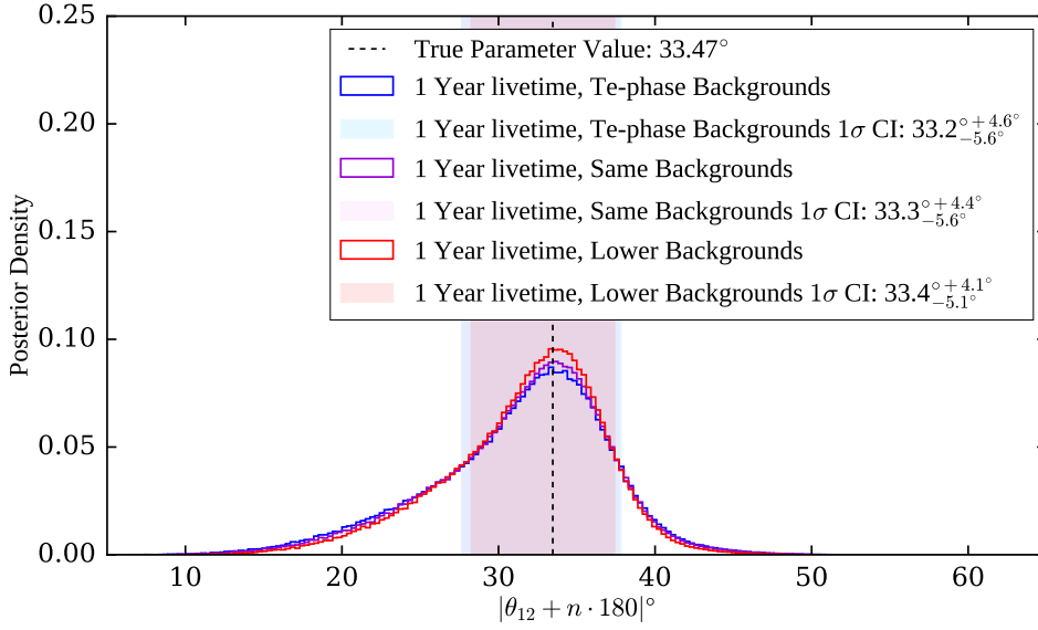
Fig. 6.25: Posterior densities marginalised onto \theta_{12} , for projections over 1 year of livetime, with different background expectations.
