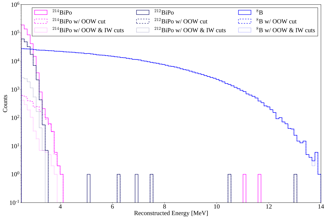
Fig. 6.8: ^{214}\text{Bi-Po} , ^{212}\text{Bi-Po} , and ^8\text{B} observed energy spectra in MC before and after OOW and IW cuts. The relative normalisations before these cuts have been applied is arbitrary.
