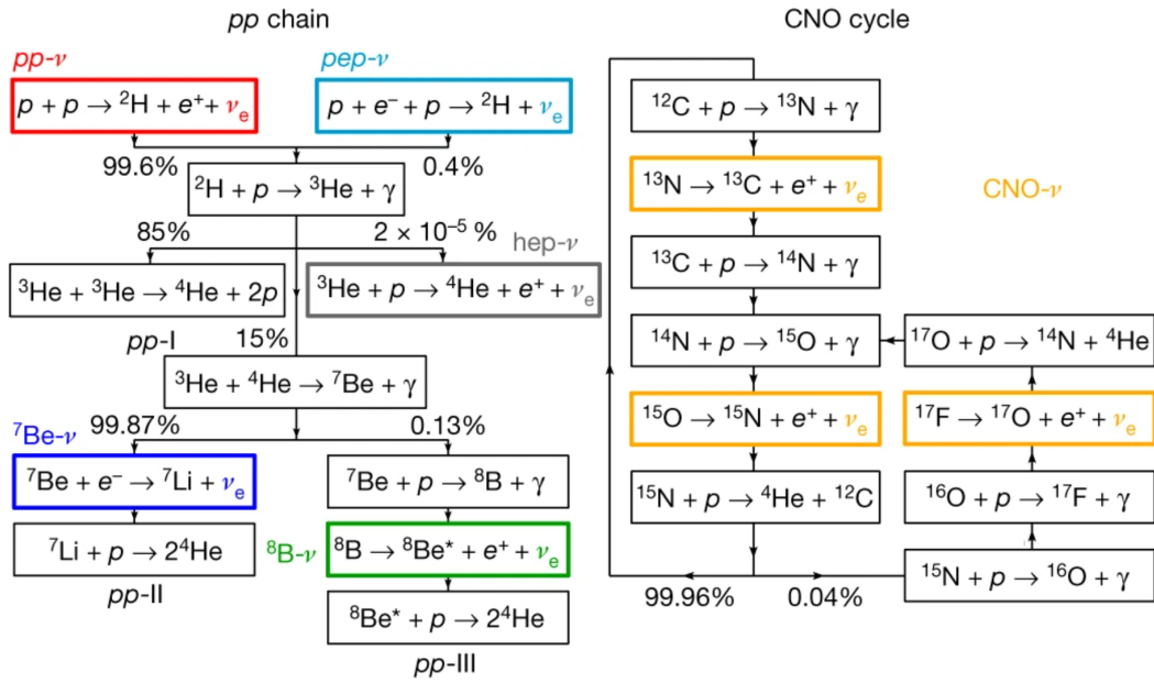
Fig. 1.1: Diagram of the pp chain and CNO cycle within the Sun, with the reactions that generate neutrinos highlighted. Taken from [29].
