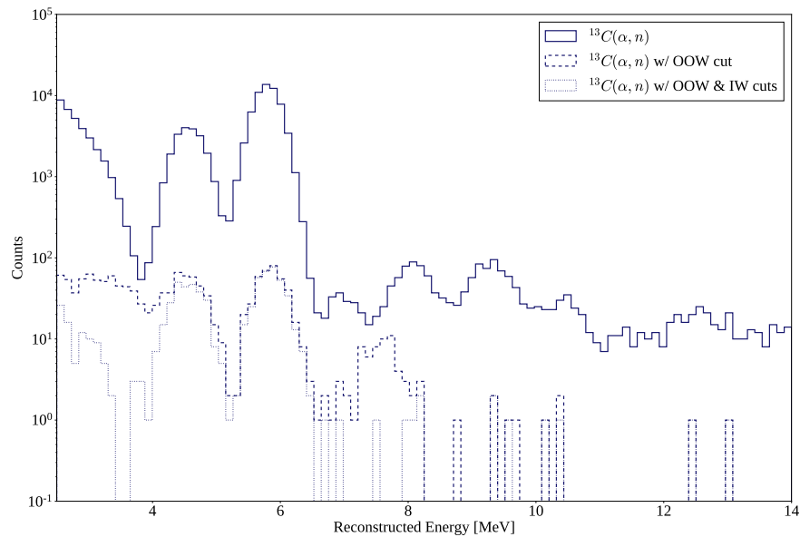
Fig. 6.10: (\alpha, n) reconstructed energy spectrum in MC within the analysis ROI, before and after out-of-window cuts have been applied. The relative normalisation of the distribution before the additional cuts have been applied is arbitrary.
