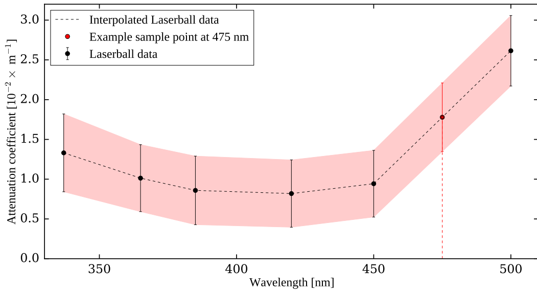
Fig. 5.3: Plot showing how linear interpolation has been used on the Laserball water phase UPW attenuation coefficient data. An example point at 475 nm is also shown.
