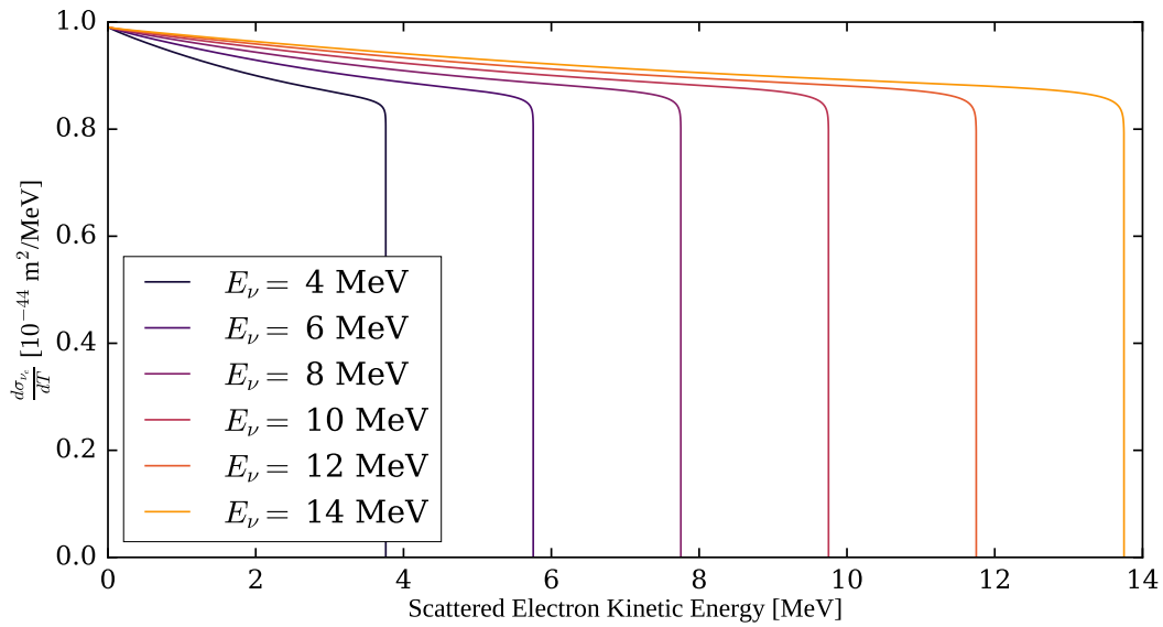
Fig. 6.2: Plot showing the differential cross-section for neutrino-electron elastic scattering of electron neutrinos, \frac{d\sigma_{\nu e}}{dT} , as a function of the kinetic energy of the scattered electron, T . This is shown for a variety of different incident neutrino energies.
