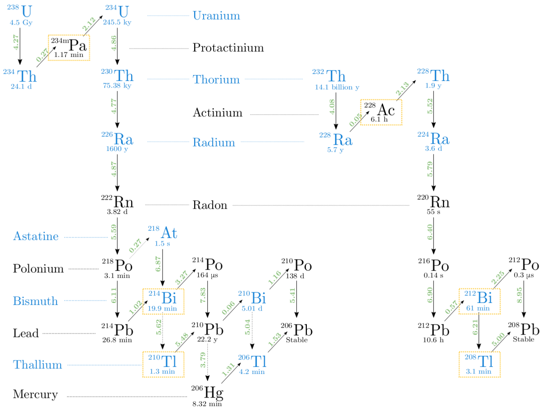
Fig. 6.6: The ^{238}\text{U} and ^{232}\text{Th} decay chains, taken from [137]. Isotopic half-lives are given below their symbol; the Q-values for each decay, in MeV, is given in green. Downward arrows indicate an \alpha -decay; diagonal arrows indicate \beta -decay. Isotopes highlighted in gold are potential backgrounds for this solar analysis.
