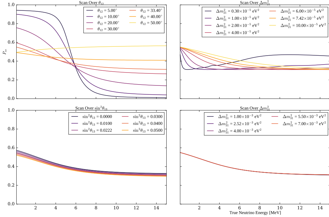
Fig. 6.1: P_{ee} as a function of true neutrino energy, scanned over a variety of oscillation parameter values. For a given oscillation parameter being scanned over, all other oscillation parameters are set at the NuFit 5.1 global fit values. P_{ee} values are calculated using the PSelmaa algorithm, as described in Section 6.3.6.
