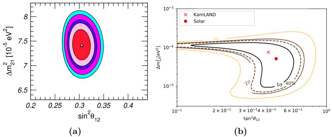
Fig. 6.5: (a): NuFit 5.1 global fit contours for the two solar neutrino oscillation parameters, after marginalisation over all other oscillation parameters [60]. Contours correspond to the allowed regions at 1\sigma , 90%, 2\sigma , 99%, and 3\sigma confidence levels. (b): Sensitivity contours produced by J. Caravaca [157] for 1 year of SNO+ data in a solar oscillation analysis sensitivity study. The analysis assumed no backgrounds, systematics, or uncertainty on the {}^8\text{B} flux. The analysis took the NuFit 4.1 ‘solar’ combined fit oscillation parameters to be true, and compared them to the reactor anti-neutrino measurement made by KamLAND [46].
