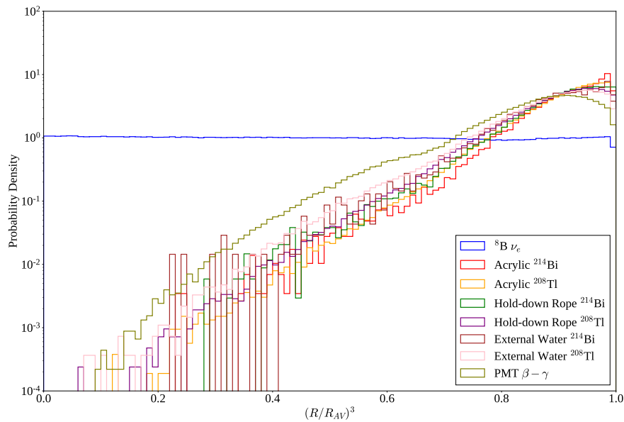
Fig. 6.11: Radial dependence of external backgrounds relevant in this analysis, as compared to the {}^8\text{B} signal. Events for all processes shown here had to pass the first 6 cuts of Table 6.2.
