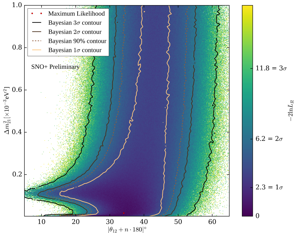
Fig. 6.19: 2D posterior density distribution marginalised onto \Delta m_{21}^2 and \theta_{12} . The colour axis shows -2 \ln L_R , proportional to the natural logarithm of the posterior density, with labels corresponding to the values associated with the N\sigma Frequentist CIs. Also shown, in shades of brown, are the Bayesian CIs.
