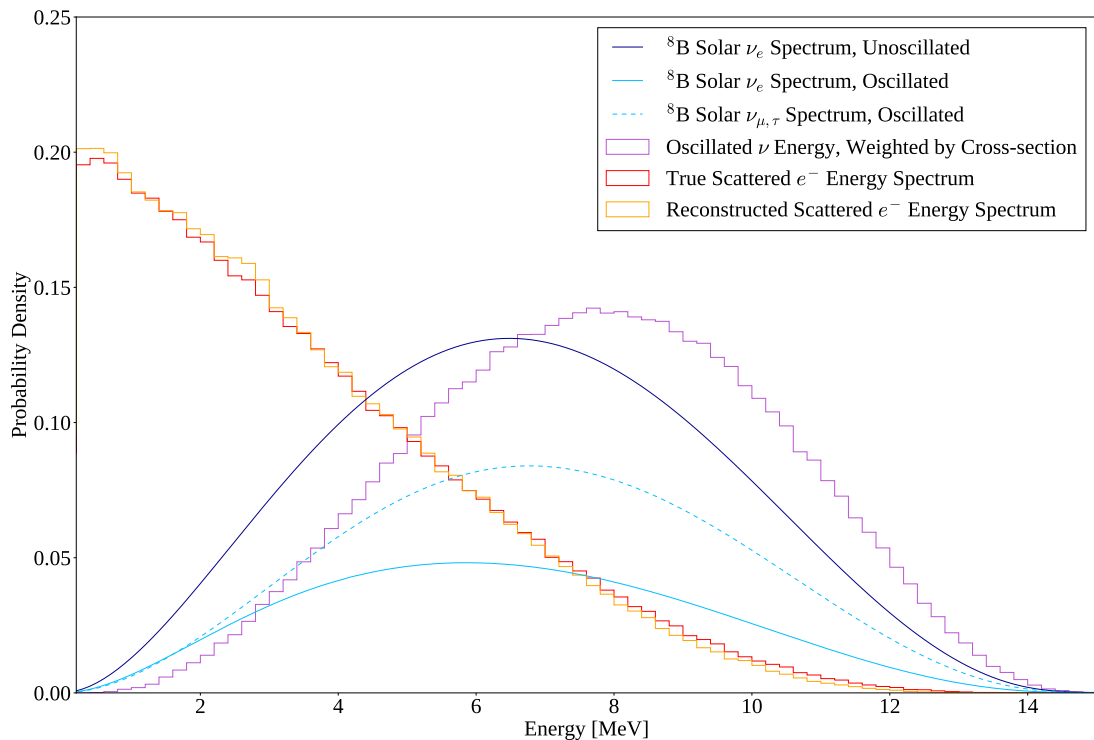
Fig. 6.3: The evolution of energy distributions related to {}^8\text{B} solar neutrino detection. The unoscillated neutrino spectrum is taken from [30]; neutrino oscillations assume oscillation parameters from the current global fit results. The latter three distributions were obtained from MC production as described in Section 6.4.1.
