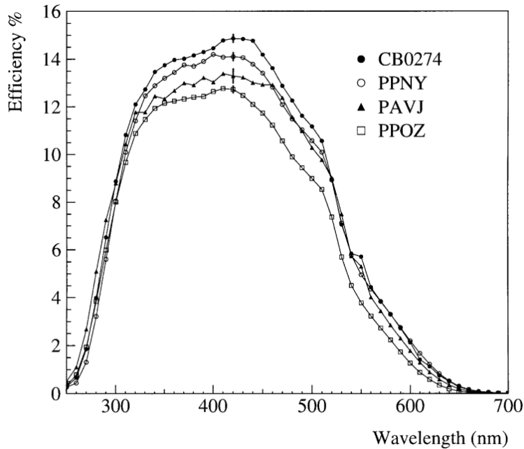
Fig. 2.8: Efficiencies of four R1408-type PMTs tested for calibration by [126].
