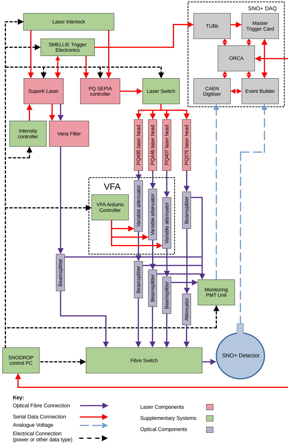
Fig. 3.3: Diagram of the connections between the various bits of SMELLIE hardware and the rest of the SNO+ detector, after the changes made in the Summer of 2022. Adapted from [115].
