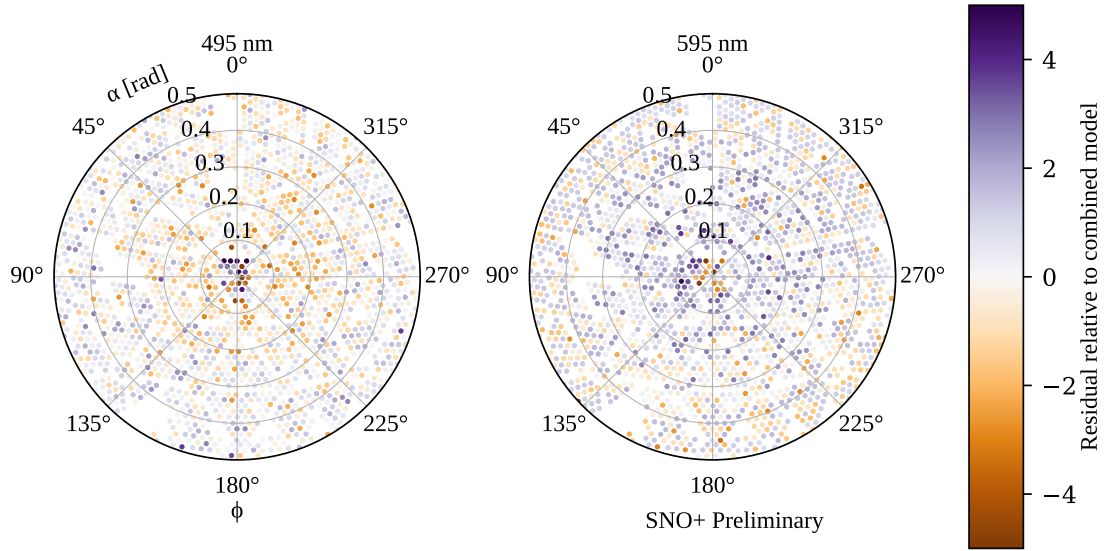
Fig. 4.9: Residuals from subruns at two different wavelengths, both compared to the combined beam profile model for fibre FS055. A positive sign, and hence bluer colours, indicate that the combined model underestimates the observed intensity for that particular subrun. Values with a magnitude beyond 5 are shown capped at this maximal value for the purposes of this plot. These PMTs are plotted in the polar fibre coordinates (\alpha, \phi) .
