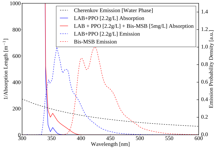
Fig. 2.2: Comparison of the SNO+ detector media’s emission and absorption properties, versus optical phase [95, 96].
