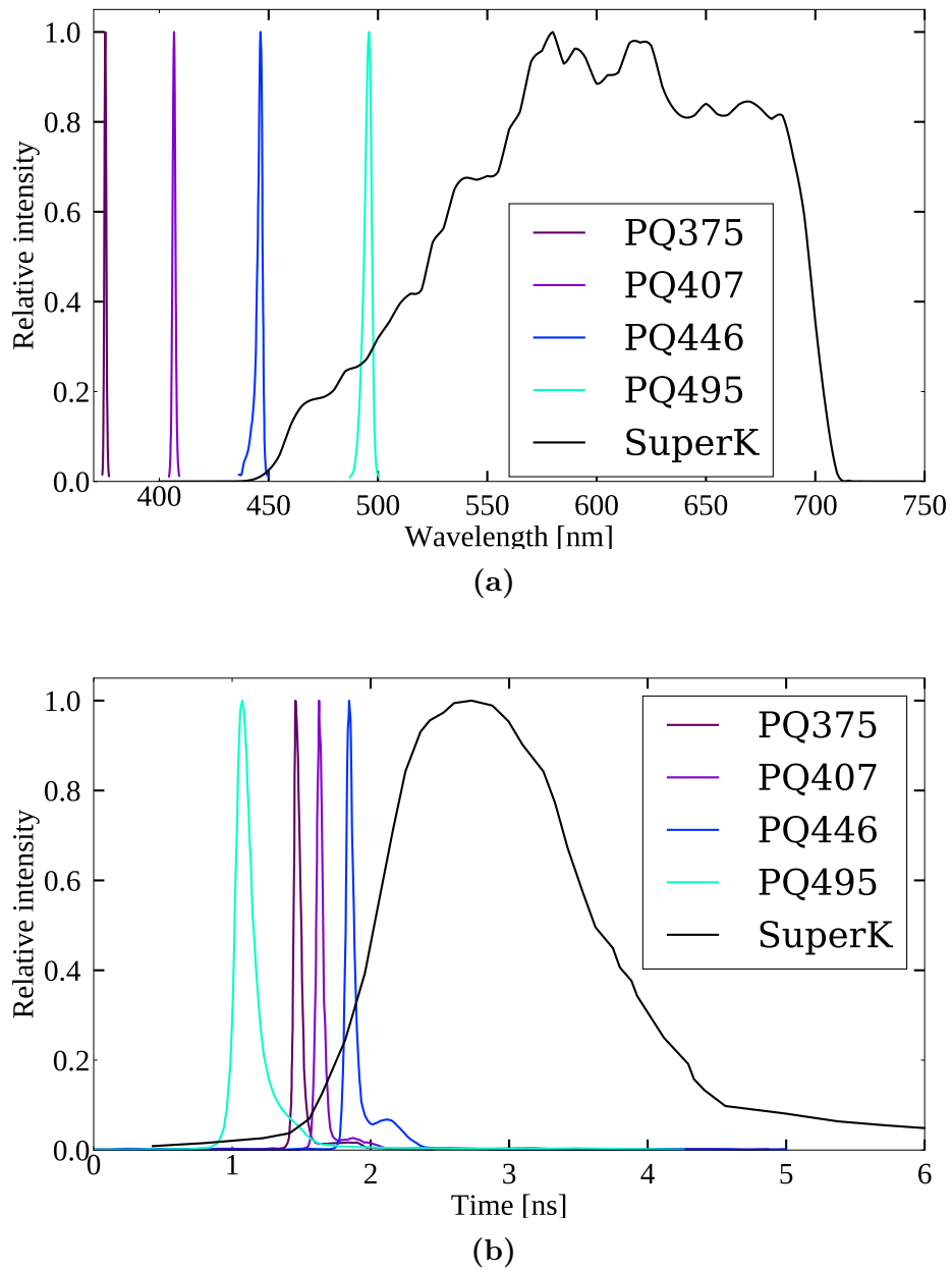
Fig. 3.4: Emission wavelength (a) and timing (b) spectra of the lasers used in SMELLIE. PQ spectral information taken from the manufacturer; SuperK information measured by J. Lidgard [142]. The SuperK wavelength spectrum shown is the full spectrum before the bandpass filter has been applied.
