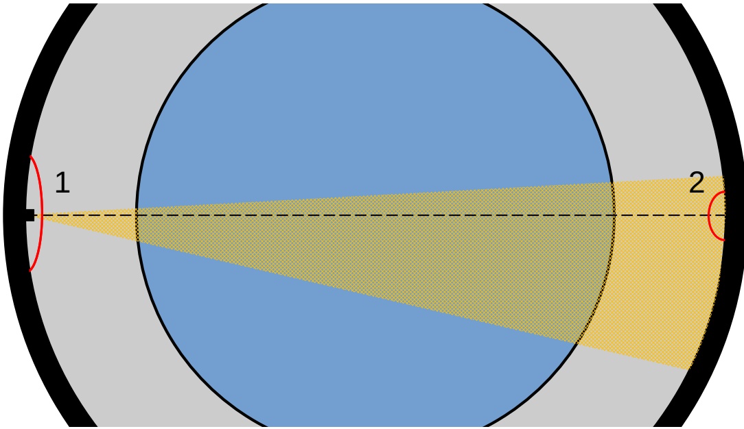
Fig. 5.2: Diagram showing the two PMT regions used in this analysis. Region 1 is the set of back-scatter PMTs, whilst region 2 is the set of far PMTs.
