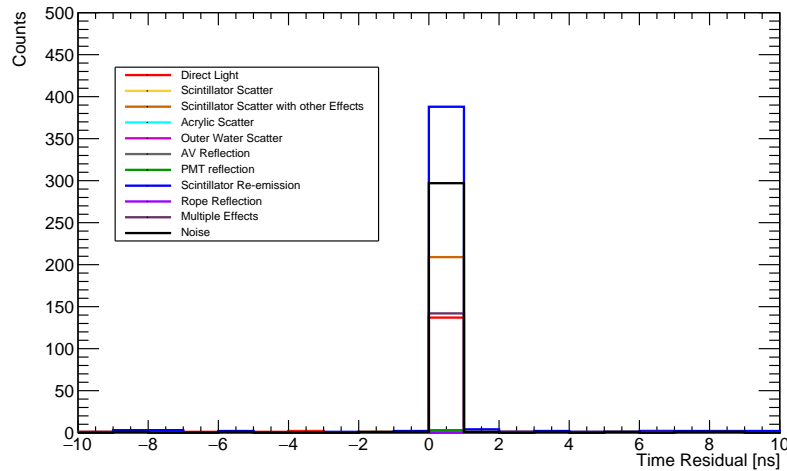
Fig. 5.6: Unstacked time residual distribution of a simulation of light from the PQ375 laser firing through fibre FS007, split by optical components. The direct light is clearly subdominant to light that has been absorbed and re-emitted by the scintillator. The spike at 0 ns arises from only one hit being observed in the beamspot for that event.
