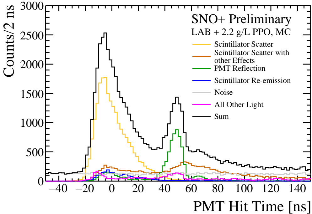
Fig. 5.14: Timing distribution of a simulation of the observed hits in the bad light-path PMT selection through fibre FS055, using the PQ495 laser. The distribution is split into the different optical components.
