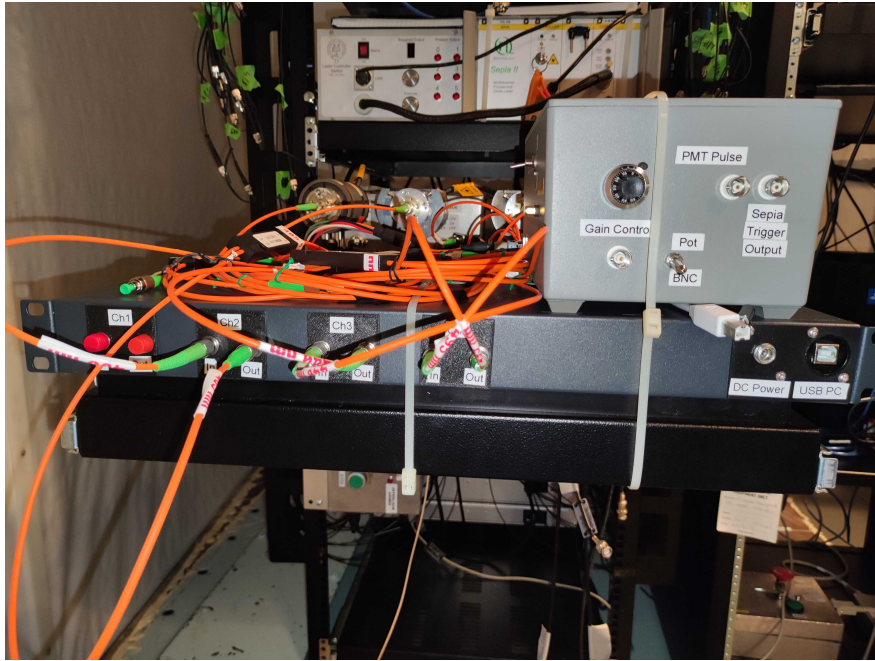
Fig. 3.7: Picture of the VFA during installation into the ELLIE hardware rack. The VFA box rests beneath the fibres connecting to the beamsplitters, as well as the newly-installed Monitoring PMT Unit (see Section 3.4 for details).
