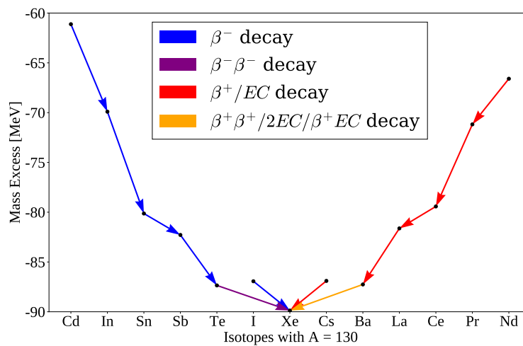
Fig. 1.6: Masses excesses of the A = 130 isobar, from [77]. The allowed weak decays between isotopes are shown by coloured arrows; note how both ^{130}\text{Te} and ^{130}\text{Ba} can only decay via second-order weak processes.
