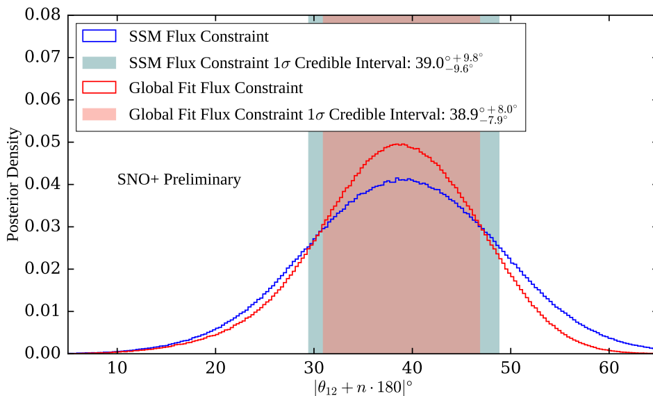
Fig. 6.20: Comparison of 1D posterior density distributions marginalised onto \theta_{12} , using both forms of ^8\text{B} flux constraint. The 1\sigma Bayesian CI are shown for both.
