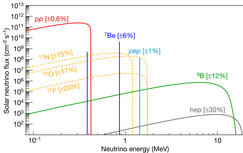
Fig. 1.2: Solar neutrino energy spectra, and associated uncertainties from the SSM. Figure is taken from [29, 31]; note that the flux is given in units of \text{cm}^{-2} \text{s}^{-1} \text{MeV}^{-1} for the continuum sources, and \text{cm}^{-2} \text{s}^{-1} for mono-energetic sources.
