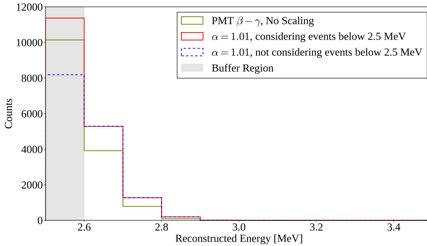
Fig. 6.13: Demonstration of how to handle an energy scaling systematic correctly. The distribution of PMT \beta - \gamma events in the analysis ROI is shown versus energy, both before and after an energy scaling of \alpha = 1.01 has been applied. If the distribution below 2.5 MeV is not known, then the scaled distribution is biased systematically. This is solved through the use of a buffer region, as indicated.
