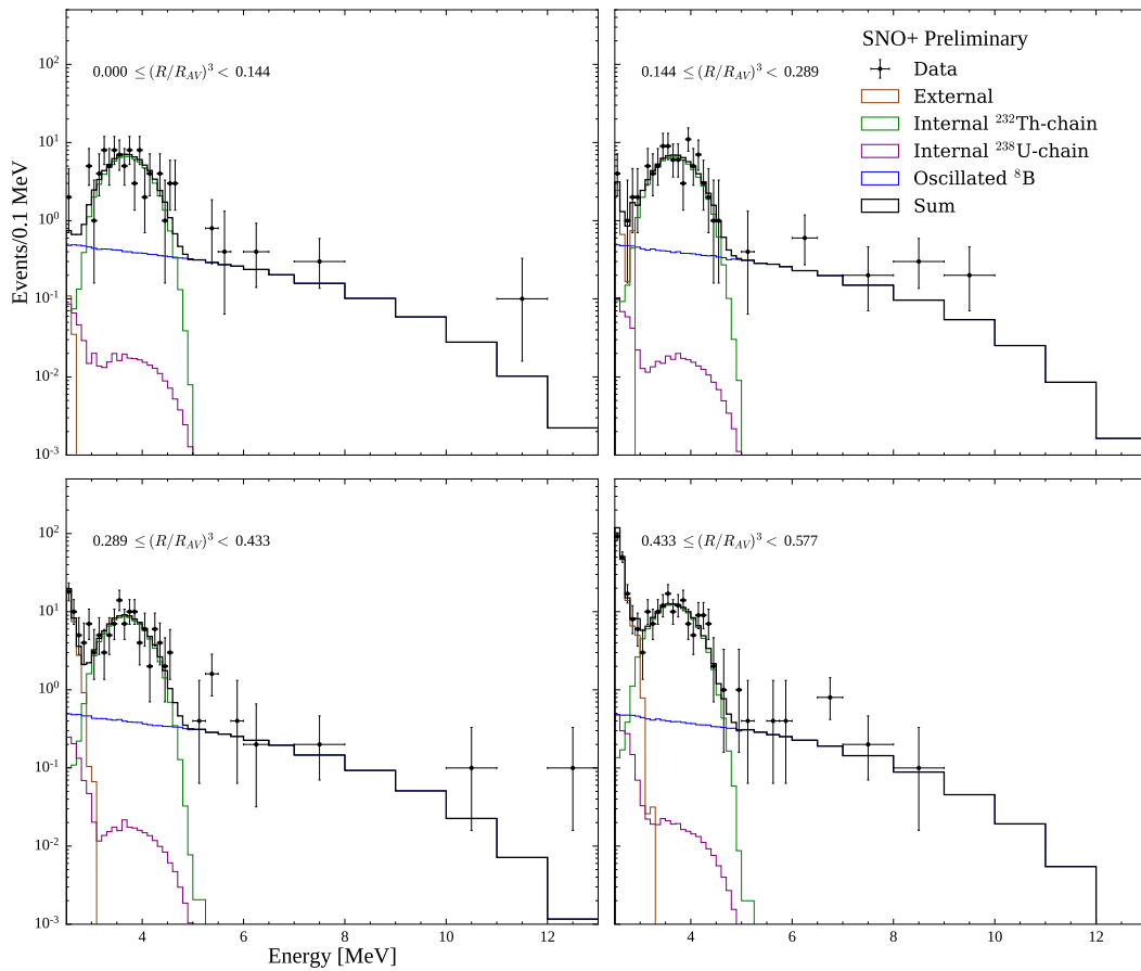
Fig. 6.21: Comparison of data to MC for each radial slice, using the best-fit parameter values derived from the MCMC results.
