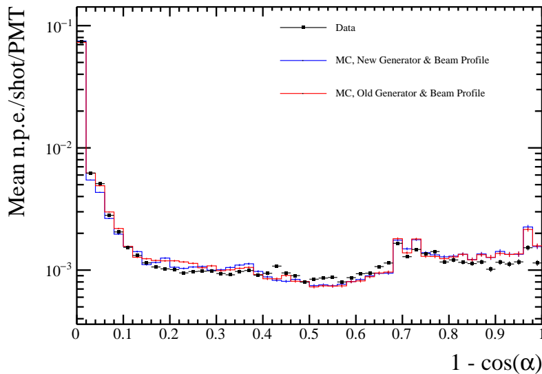
Fig. 4.5: Comparison of water-phase data to MC generated using both the old and new 2D beam profile generator approaches. The new generator also uses the updated beam profiles, as discussed in Section 4.2. The MC distributions have been scaled to match the total npe of the data.
