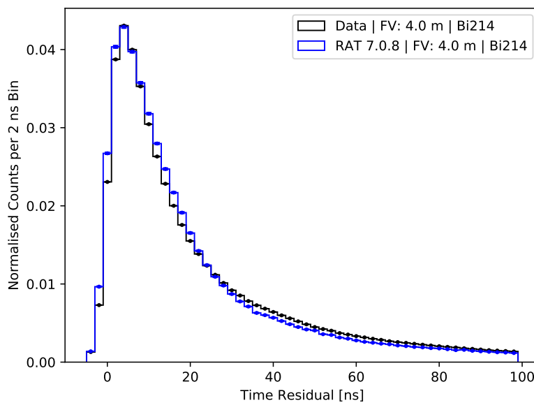
Fig. 2.3: Comparison between the observed emission time distribution of electrons from tagged ^{214}\text{Bi} \beta -decays and a production of matching simulated events, after fitting the timing constants. Adapted from [98]. “FV” corresponds to the Fiducial Volume used in this plot; “RAT 7.0.8” is the version of the simulation software used to compare to data.
