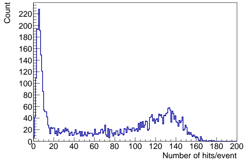
Fig. 3.6: Distribution of the number of PMT hits observed per event in the detector for laser PQ446 when the driving voltage value was 280. Data taken on February 22 nd , 2021.
