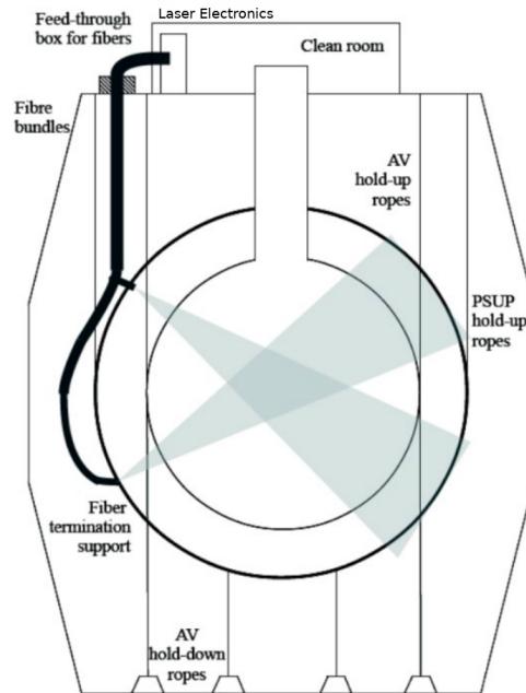
Fig. 3.1: Diagram of the SMELLIE calibration system within SNO+. Modified from [138].
