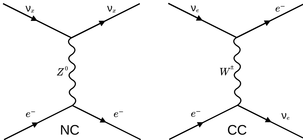
Fig. 1.3: The tree-level Feynman diagrams associated with the NC and CC modes of neutrino-electron elastic scattering.
