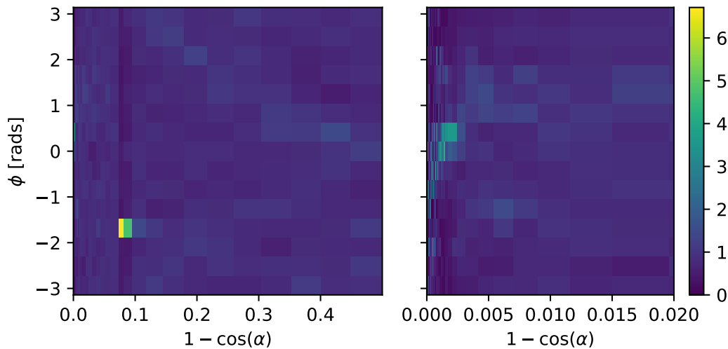
Fig. 4.4: Histogram of interpolated intensities within the 2D direction-space. The left view shows the full histogram; the right is a zoomed-in version near the beamspot. Unlike the binning in \phi , the bin widths in r are not at all uniform. Instead, they have been determined such that the area summed over a given “strip” of bins of constant r will be the same.
