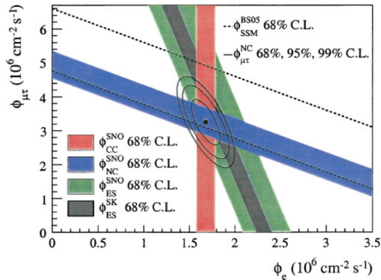
Fig. 1.4: Measured solar neutrino fluxes from electron neutrinos versus muon and tau neutrinos, in the SNO CC, NC, and ES modes (coloured bands). Also shown is the expectation from the SSM (dotted lines), and the ES rate measured from Super-Kamiokande (black band). The combined probability contours are shown in black. Taken from [41].
