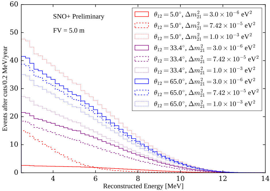
Fig. 6.4: Comparison of the reconstructed electron energy distribution expected for 9 different oscillation parameter combinations, after 1 year of data. The unoscillated rate was calculated in Appendix A, with the cuts described in Section 6.4.2 being applied.
