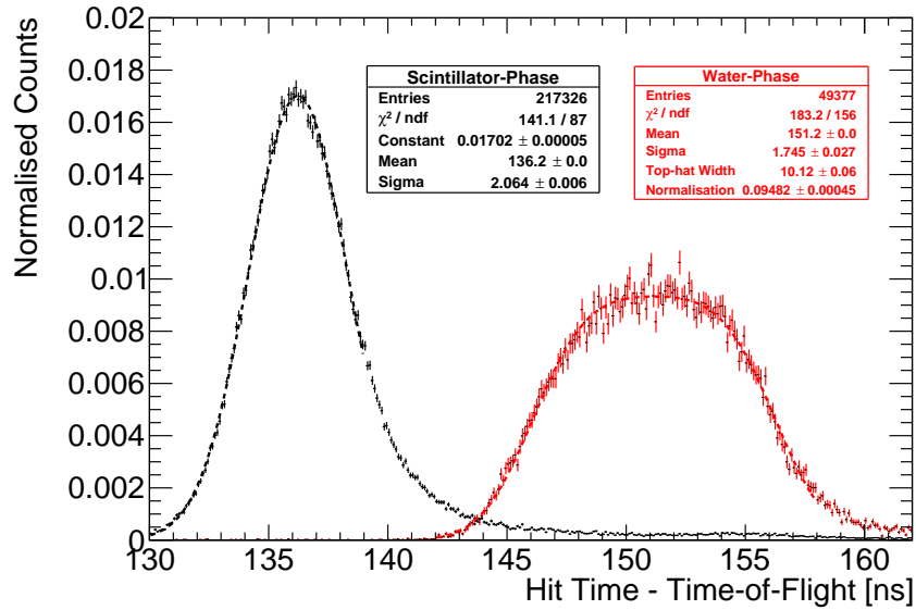
Fig. 3.13: Comparison of observed hit times in beamspot for laser PQ495 through fibre FS007, before and after T. Zummo’s firmware update to TUBii. The initial data was taken by E. Turner June 20 th 2018 during the water phase, whilst the data post-fix was taken by myself on June 24 th 2023 during the scintillator phase. The peak of the former is fit to the convolution of a Gaussian with a top-hat function, whilst the latter is just fit with a Gaussian function.
