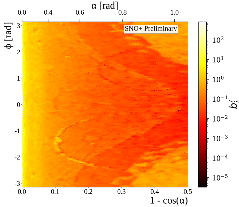
Fig. 4.8: Interpolated intensity map for the new updated beam profile of fibre FS055. The misalignment of rope shadows and AV effects, can both be seen.
