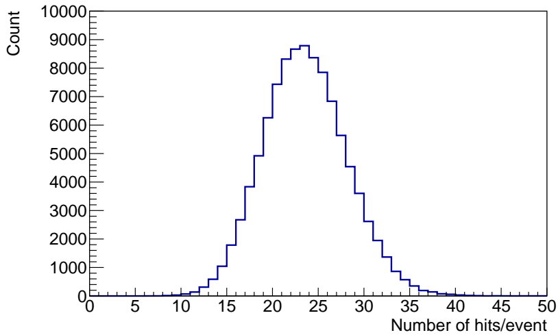
Fig. 3.9: Distribution of the number of PMT hits observed per event in the detector for laser PQ446, for a subrun of data taken in June 2023 after the VFA has been installed.
