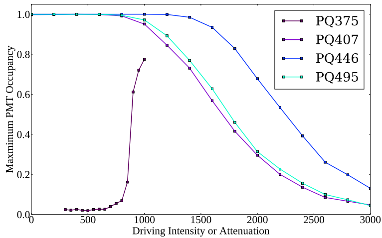
Fig. 3.8: Maximum occupancy in the detector as a function of the attenuation parameter value used, for each of PQ407, PQ446, and PQ495. Because PQ375 is not plugged into the VFA, its dependence on the driving intensity is shown instead. Data taken on the 12 th of January, 2023.
